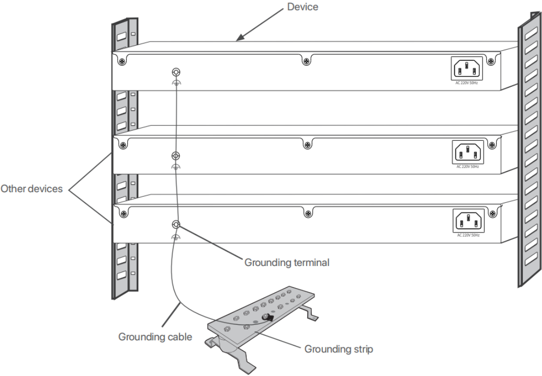
Figure 2-4 Equipotential bonding connection
