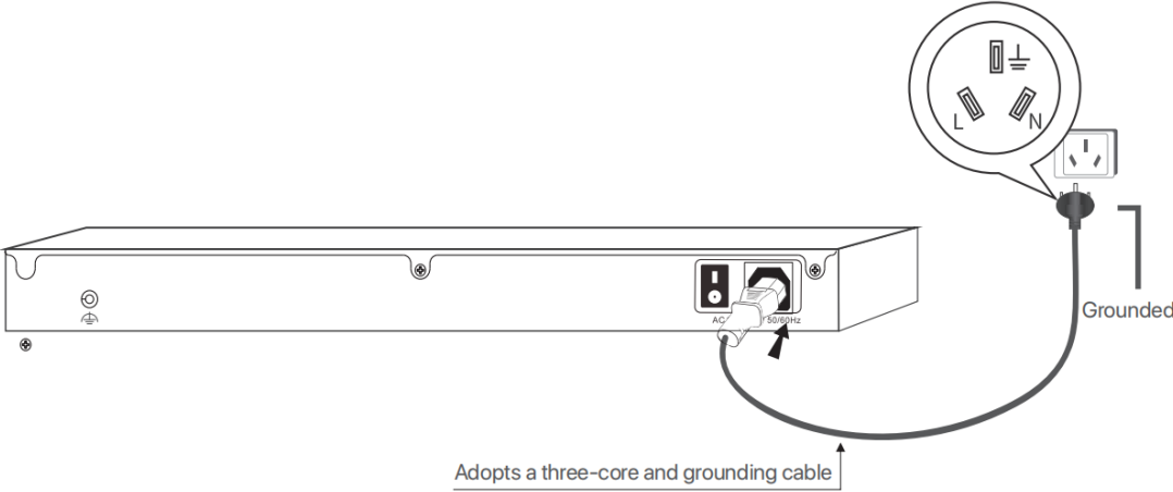
Figure 2-3 Grounding through an PE wire
