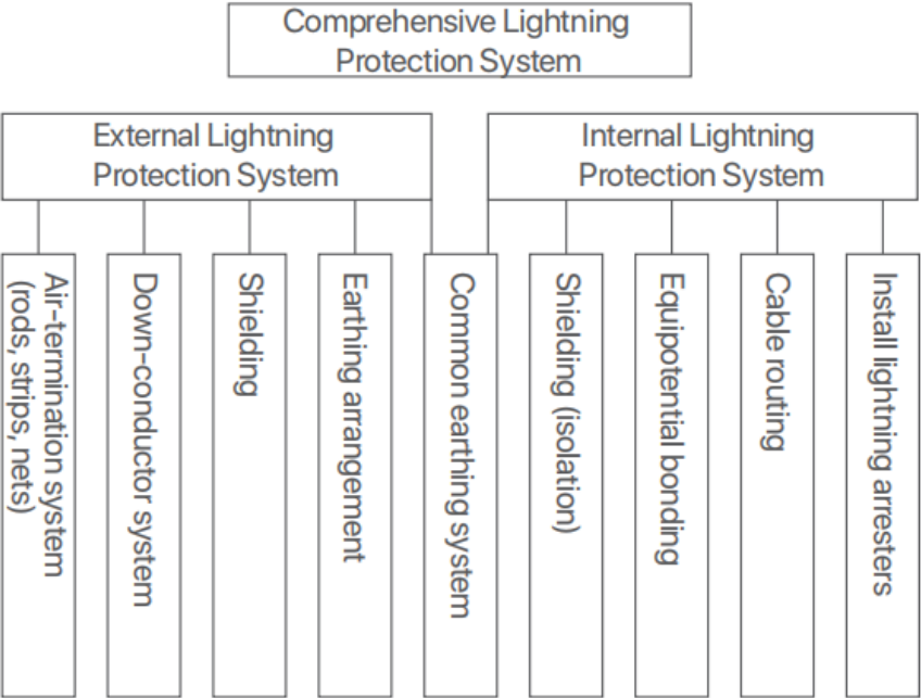
Figure1-1 Comprehensive lightning protection system
