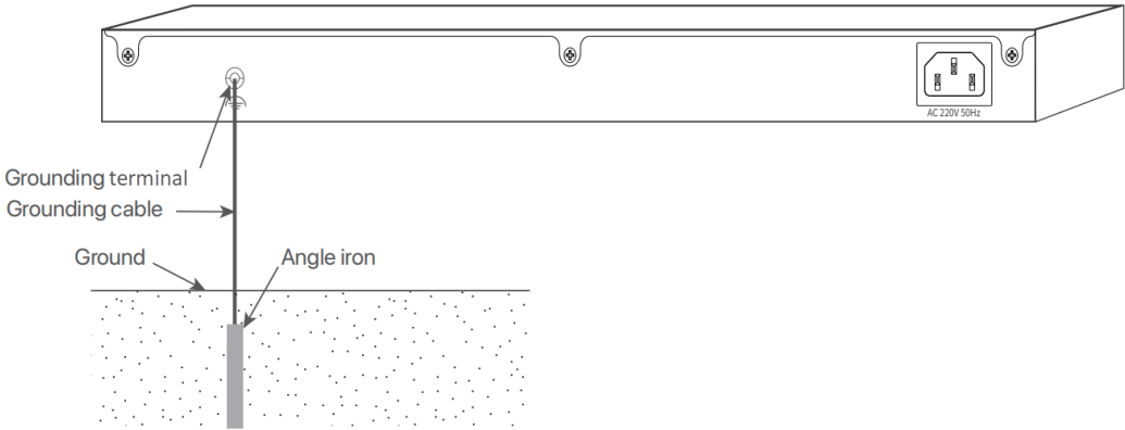
Figure 2-2 Grounding installation (the grounding conductor buried near the equipment room)
