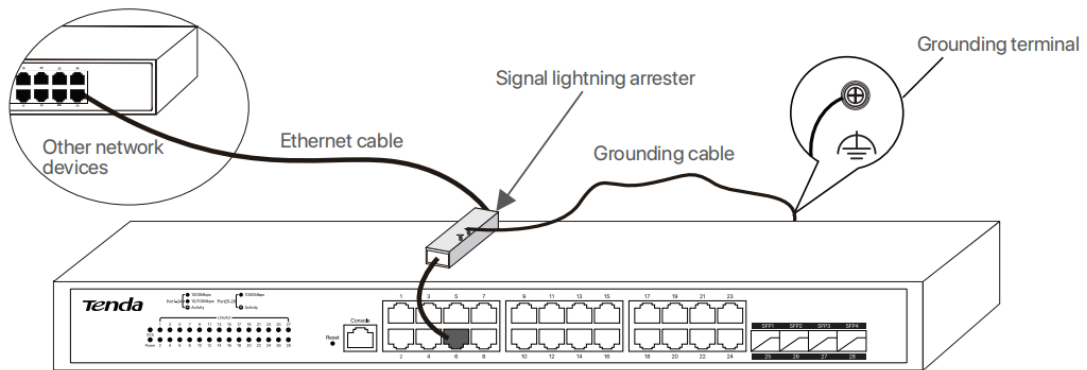
Figure 3-1 Connect a signal lightning arrester
